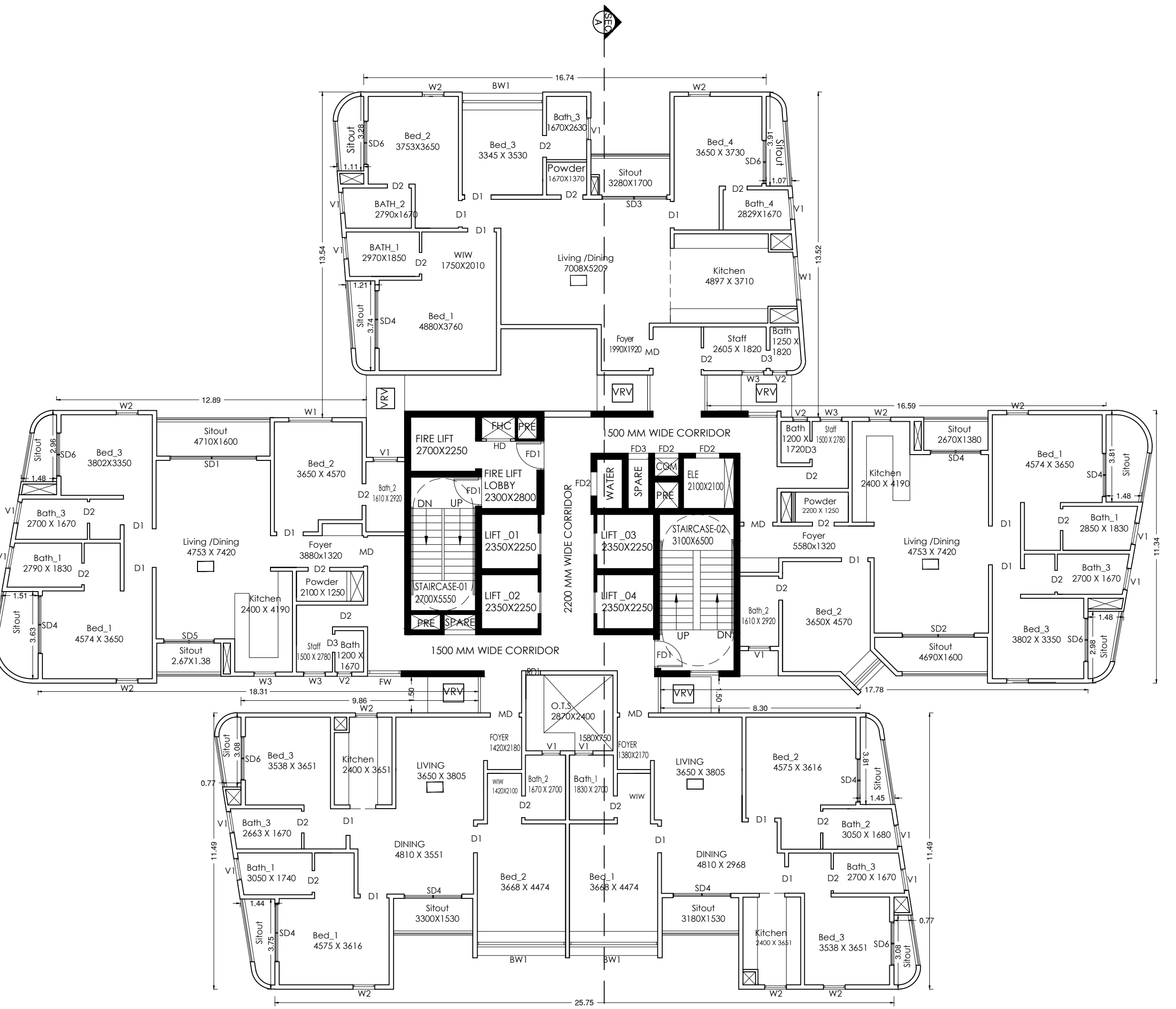
TOWER - A TYPICAL 4th to 6th, 8th, 8th to 10th, 12th to 14th, 16th, 18th, 20th to 22nd, 24th, 25th, 28th & 29th FLOOR PLAN NO OF UNITS (05 X 16) = 80 Units
