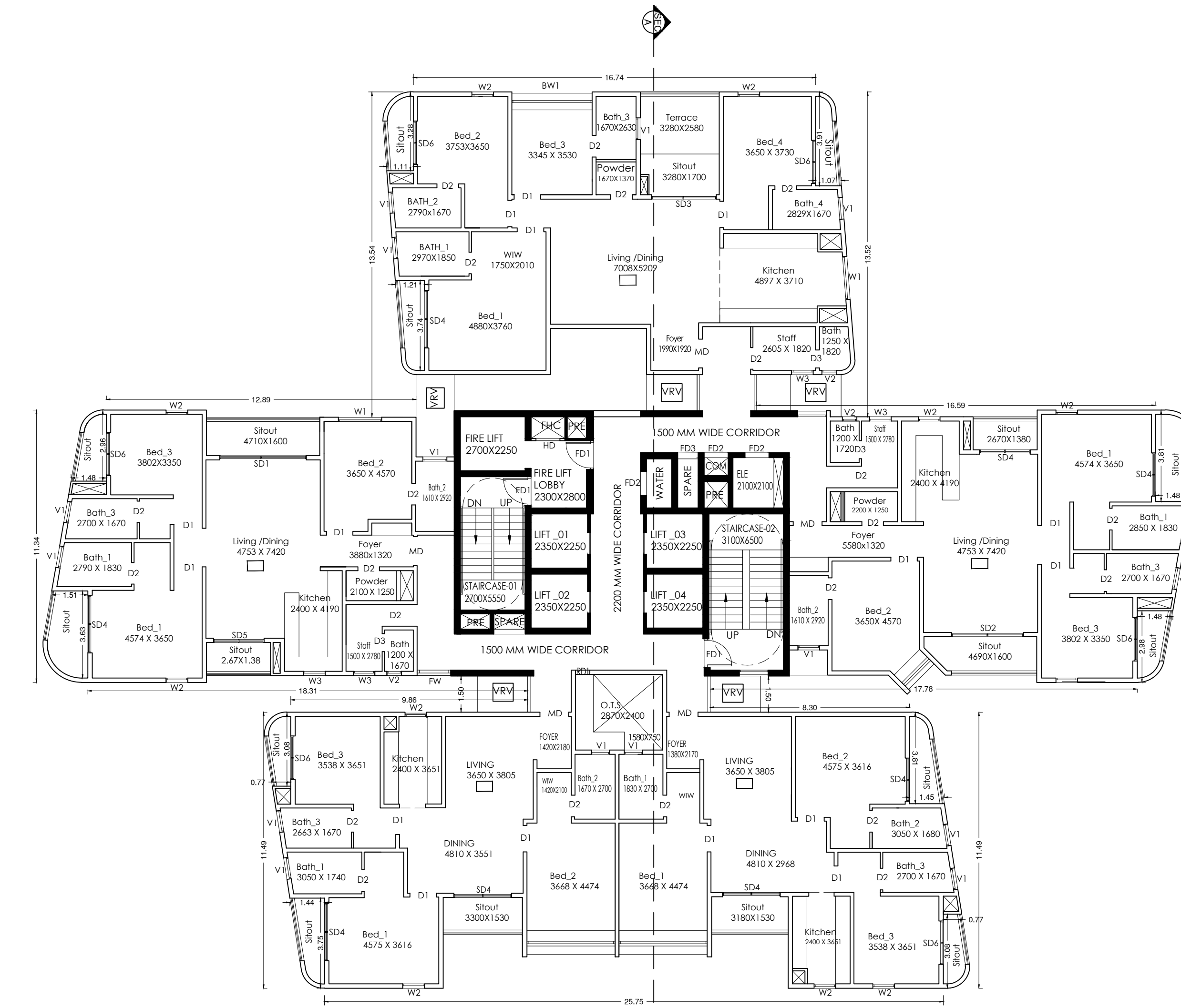
TOWER - A TYPICAL 17th & 26th FLOOR PLAN NO OF UNITS (05 X 02) = 10 Units
