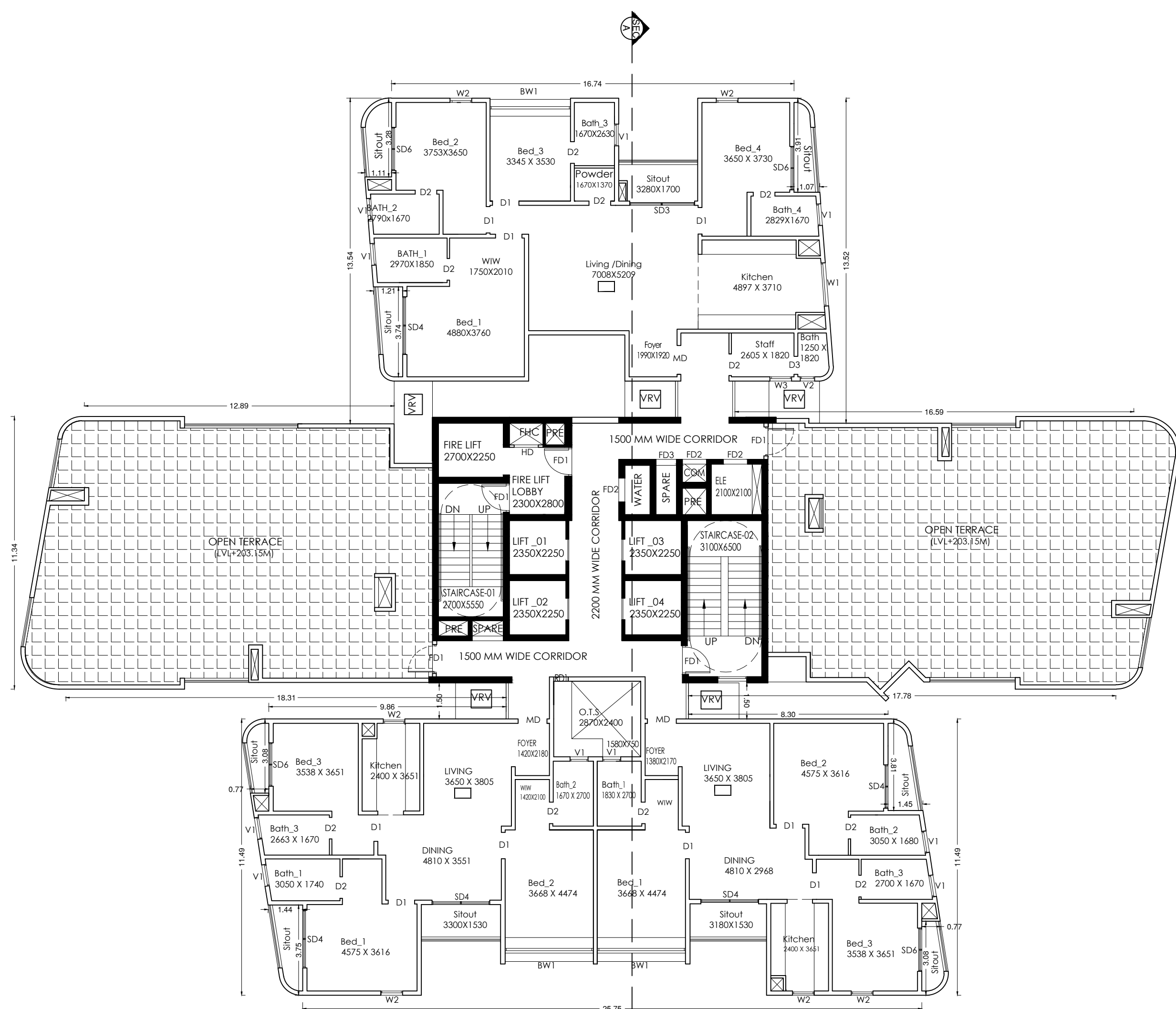
TOWER - A 3rd FLOOR PLAN NO OF UNITS - 05 Units (LV-1+14.50M)
